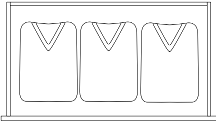
larghezza mm 941 width 37" interno utile cassetto l 869 p 436 h 95-178 useful drawer interior w 34 1/4" d 17 1/4" h 3 3/4"-7"
