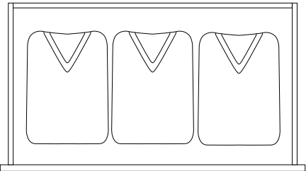
larghezza mm 941 width 37" interno utile cassetto l 809 p 435,5 h 113-264 interno utile vassoio l 813 p 435 h 105 useful drawer interior w 31 3/4" d 17 1/4" h 4 1/2"-10 1/2" useful tray interior w 32" d 17 1/4" h 4 1/4"
