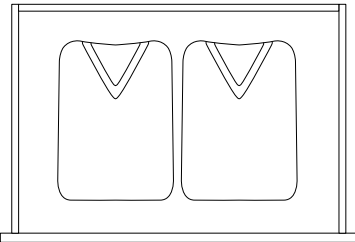
larghezza mm 780 width 30 3/4" interno utile cassetto l 648 p 435,5 h 113-264 interno utile vassoio l 652 p 435 h 105 useful drawer interior w 25 1/2" d 17 1/4" h 4 1/2"-10 1/2" useful tray interior w 25 3/4" d 17 1/4" h 4 1/4"
