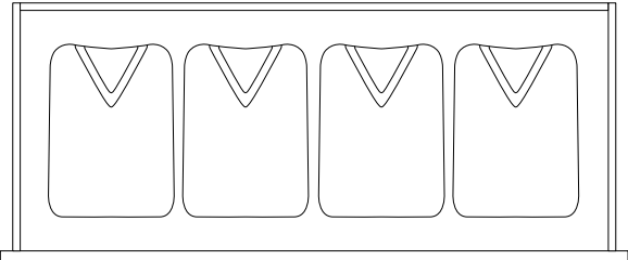
larghezza mm 1263 width 49 3/4" interno utile cassetto l 1131 p 435,5 h 113-264 interno utile vassoio l 1135 p 435 h 105 useful drawer interior w 44 1/2" d 17 1/4" h 4 1/2"-10 1/2" useful tray interior w 44 3/4" d 17 1/4" h 4 1/4"
