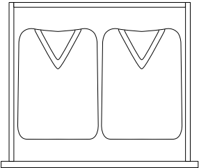
larghezza mm 619 width 24 1/4" interno utile cassetto l 487 p 435,5 h 113-264 interno utile vassoio l 491 p 435 h 105 useful drawer interior w 19 1/4" d 17 1/4" h 4 1/2"-10 1/2" useful tray interior w 19 1/4" d 17 1/4" h 4 1/4"
