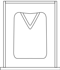
larghezza mm 458 width 18" interno utile cassetto l 326 p 435,5 h 113-264 useful drawer interior w 12 3/4" d 17 1/4" h 4 1/2"-10 1/2"
